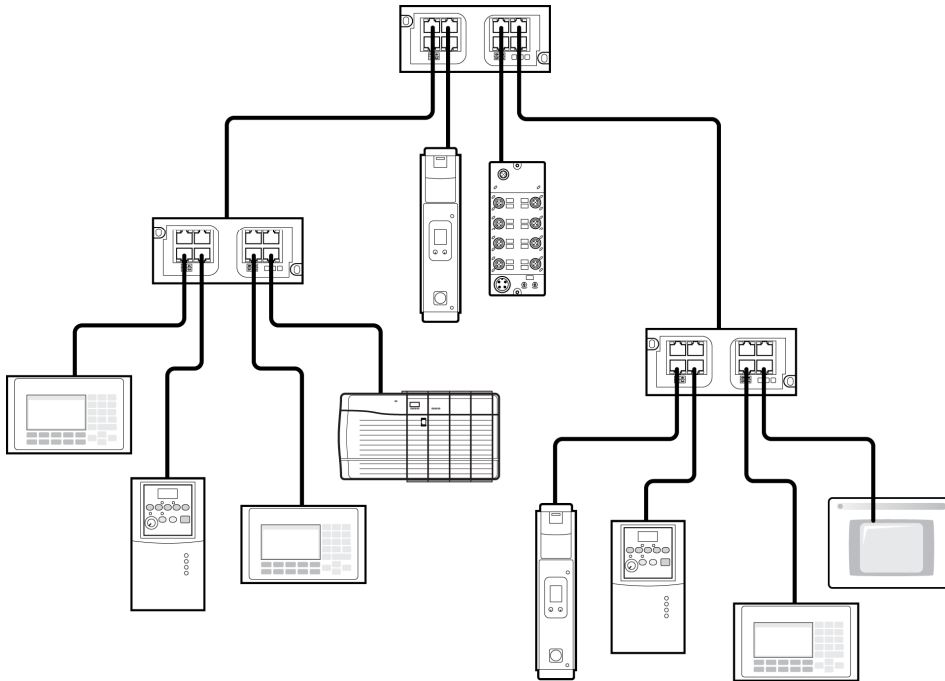
Figure 7 Hierarchal Star
