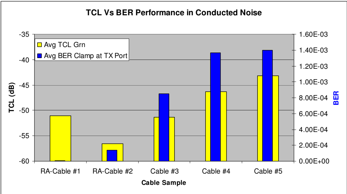
Figure 17 BER Performance VS TCL
