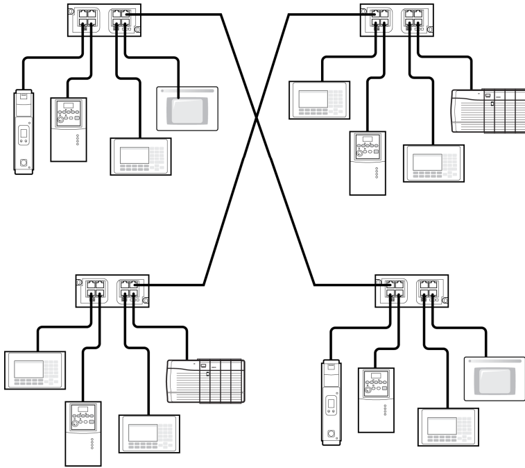
Figure 8 Spanning Tree
